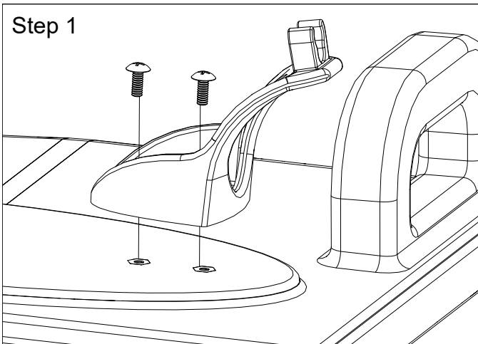
Step 1 Attach the (2) Hose Wraps to the top of the tank with (4) Phillips Head Screws
