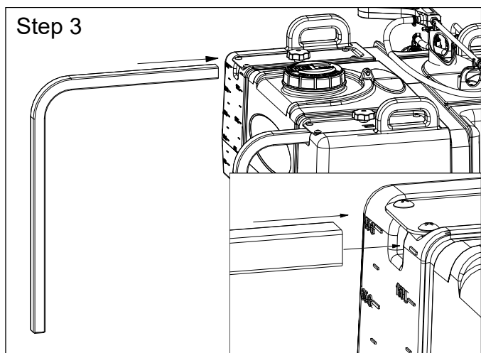
Step 3 With the unit in a UTV Box, slide the boom mount tubes in to the tank mounts and tighten the lobe knob.
