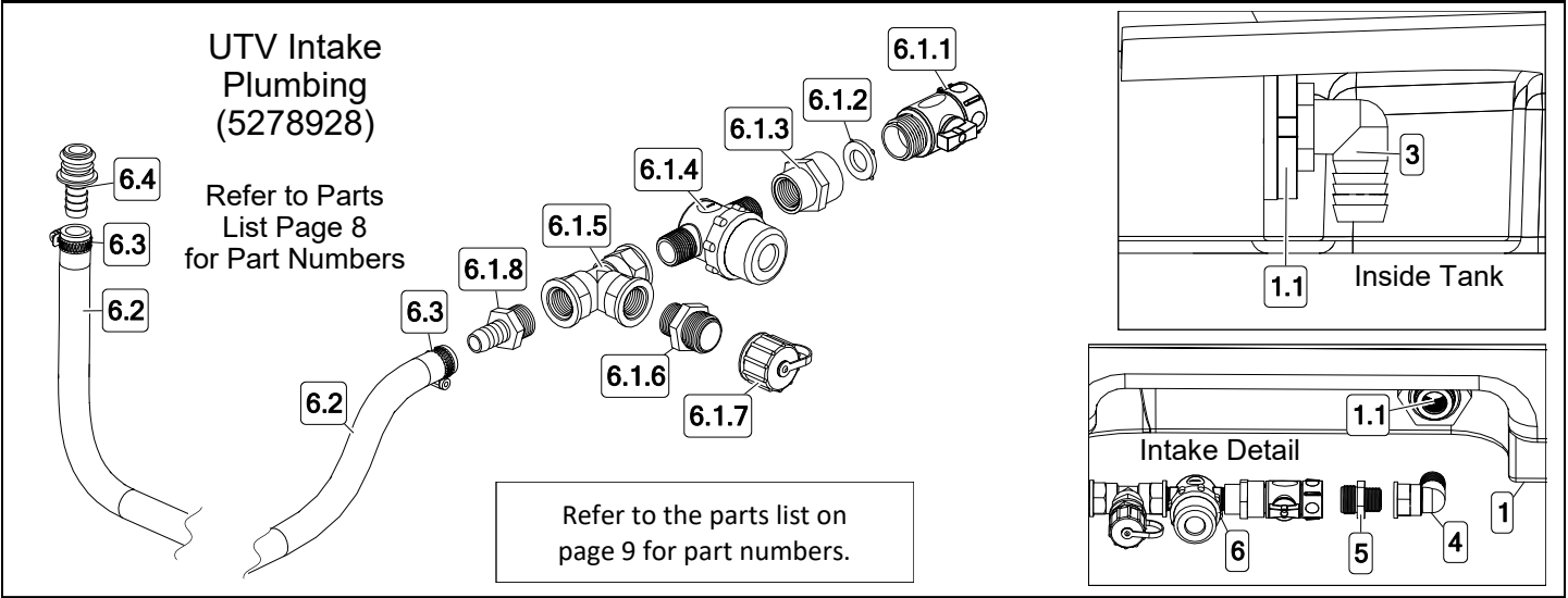
Boomless “Wet” Boom Assembly Exploded View/Parts List (5275260)
