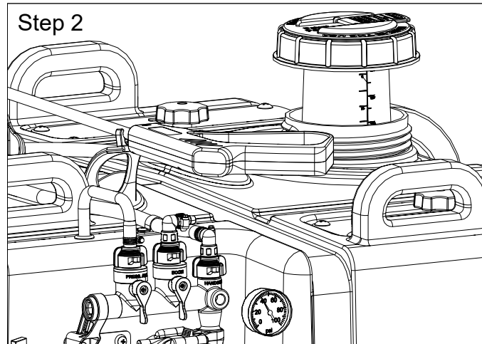
Step 2 Thread Pressure Gauge into open port on manifold., as shown.
