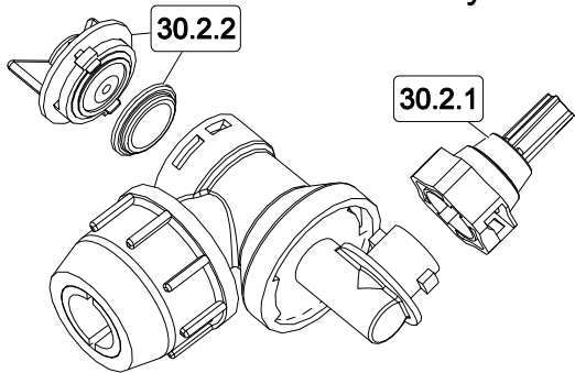
End Nozzle Assembly
