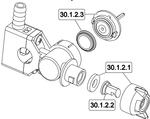
Center Nozzle Assembly
